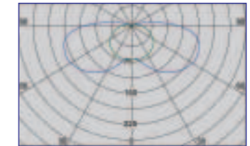
Typical Polar Curve of 2050
